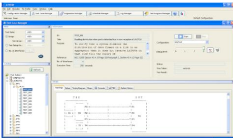
Figure 2: Testcase Manager
