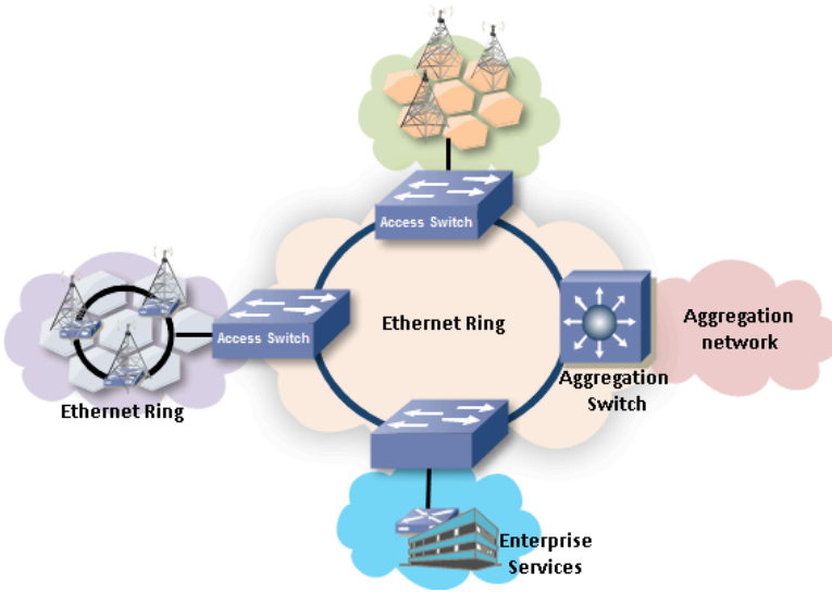
Figure 1. Ethernet Ring Protection Switching in Mobile Backhaul
