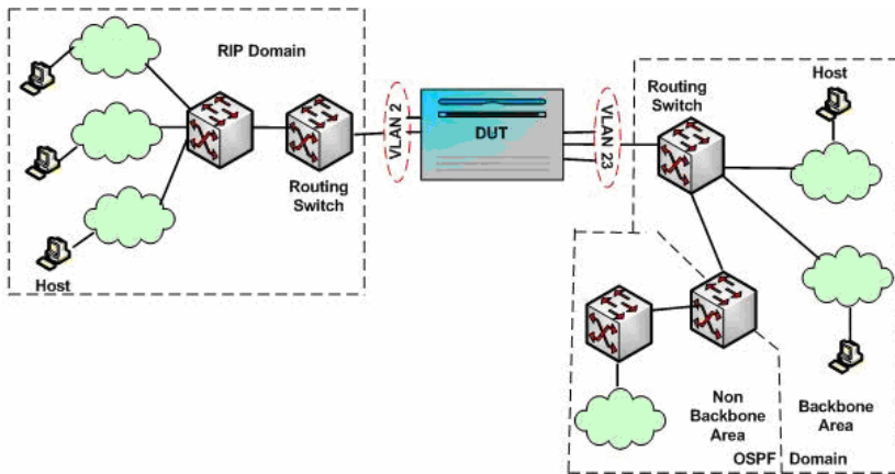
Figure 1. A Sample Multiple IGP-based IPv4 Test Topology
